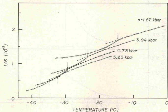
Fig. 2. Temperature dependence of the inverse dielectric constant along the c^* -direction of (\text{NH}_4)_3\text{H}(\text{SO}_4)_2 at various hydrostatic pressures. The anomaly at the II-III transition is indicated by the vertical arrows.
